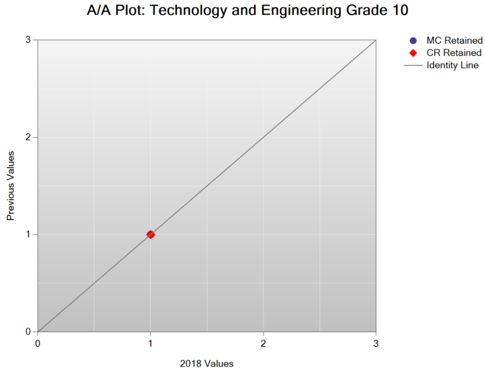
Figure K-11. 2018 Legacy MCAS: \alpha -Plot –Technology and Engineering Grade HS
