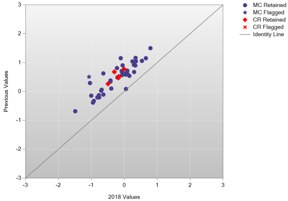
B/B Plot: Introductory Physics Grade 10
