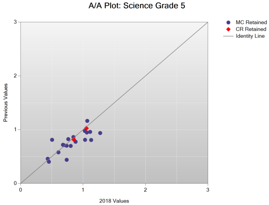
Figure K-13. 2018 Legacy MCAS: \alpha -Plot –Science Grade 5
