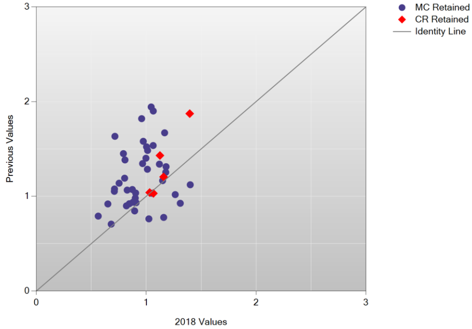
Figure K-8. 2018 Legacy MCAS: b -Plot –Chemistry Grade HS
