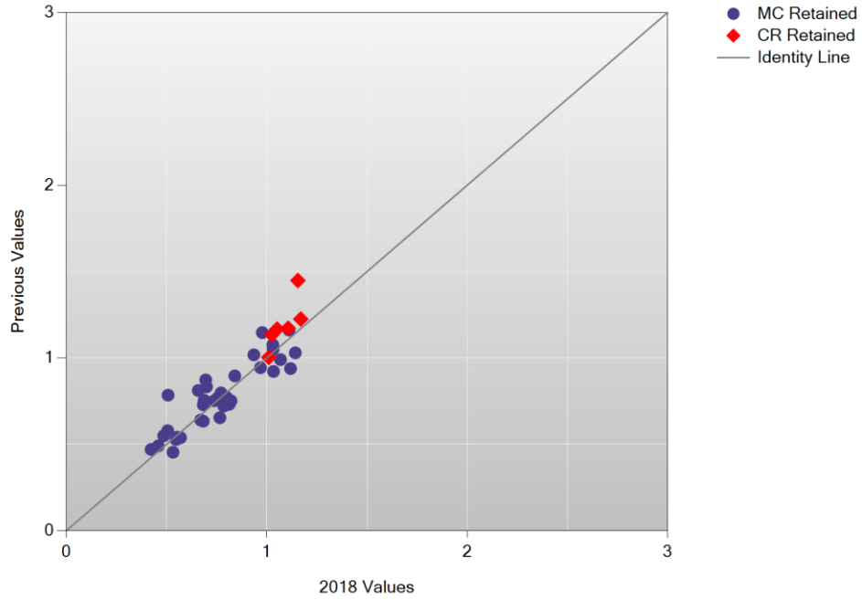
Figure K-2. 2018 Legacy MCAS: b -Plot –ELA Grade 10
