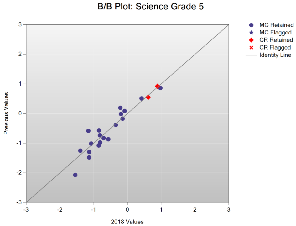
Figure K-14. 2018 Legacy MCAS: b -Plot –Science Grade 5
