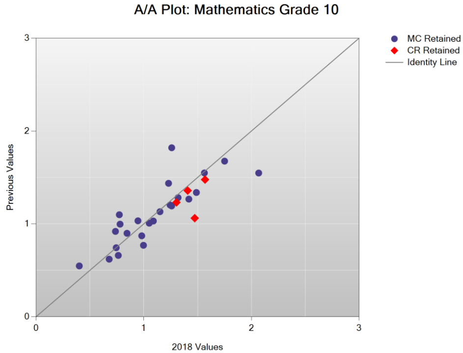
Figure K-3. 2018 Legacy MCAS: \alpha -Plot –Mathematics Grade 10
