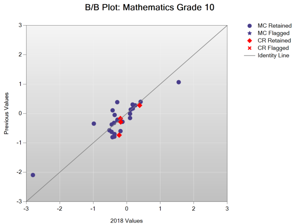
Figure K-4. 2018 Legacy MCAS: b -Plot –Mathematics Grade 10
