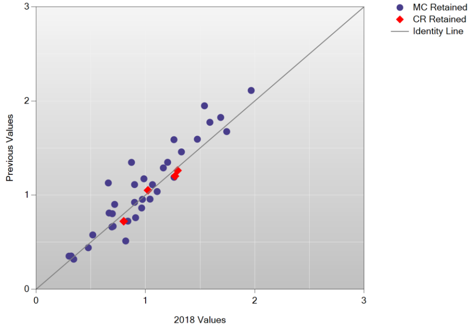
Figure K-6. 2018 Legacy MCAS: b -Plot –Biology Grade HS
