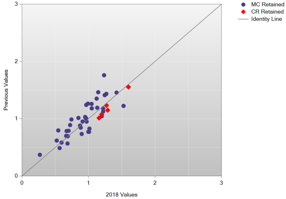
A/A Plot: Introductory Physics Grade 10
